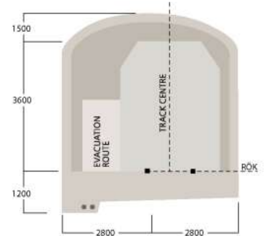
SINGLE-TRACK TUNNEL Rock cross section: 26 m 2
