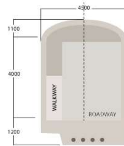
SERVICE TUNNEL Rock cross section: 26 m 2
