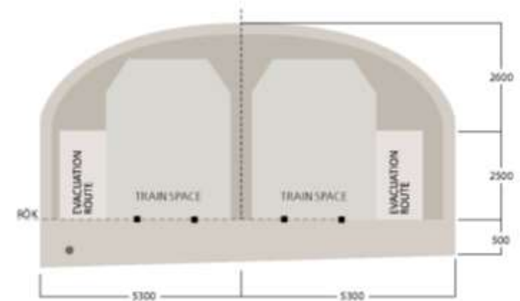
DOUBLE-TRACK TUNNEL Rock cross section: 58 m 2
