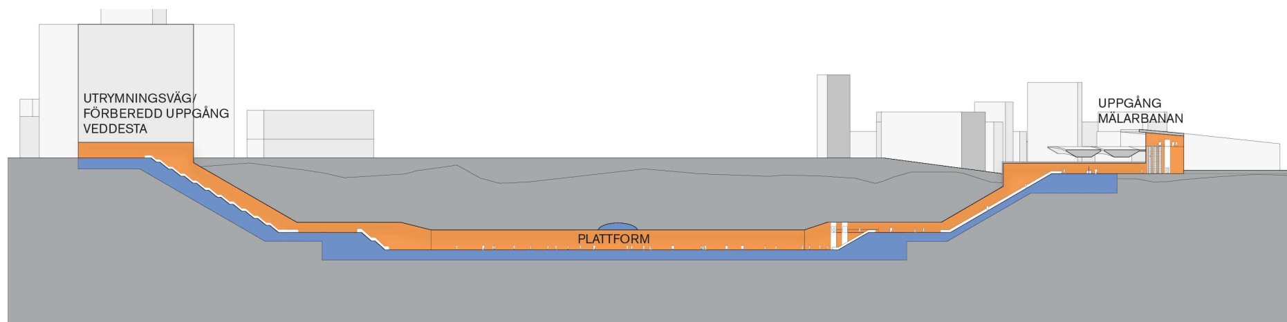
Figur 4.16 Barkarby station i profil.
